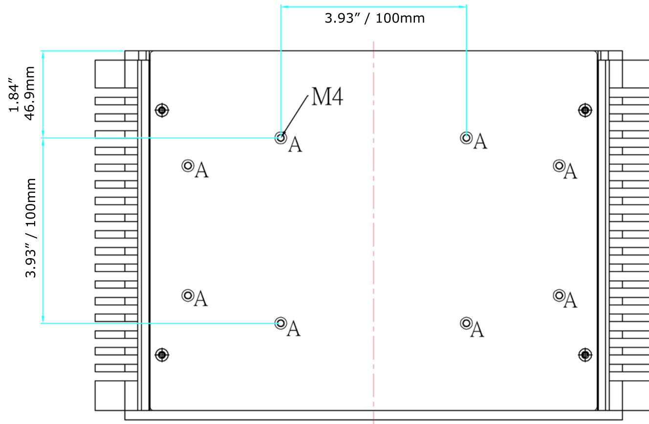
Bottom View, VESA Mounting
