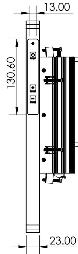
Right View
