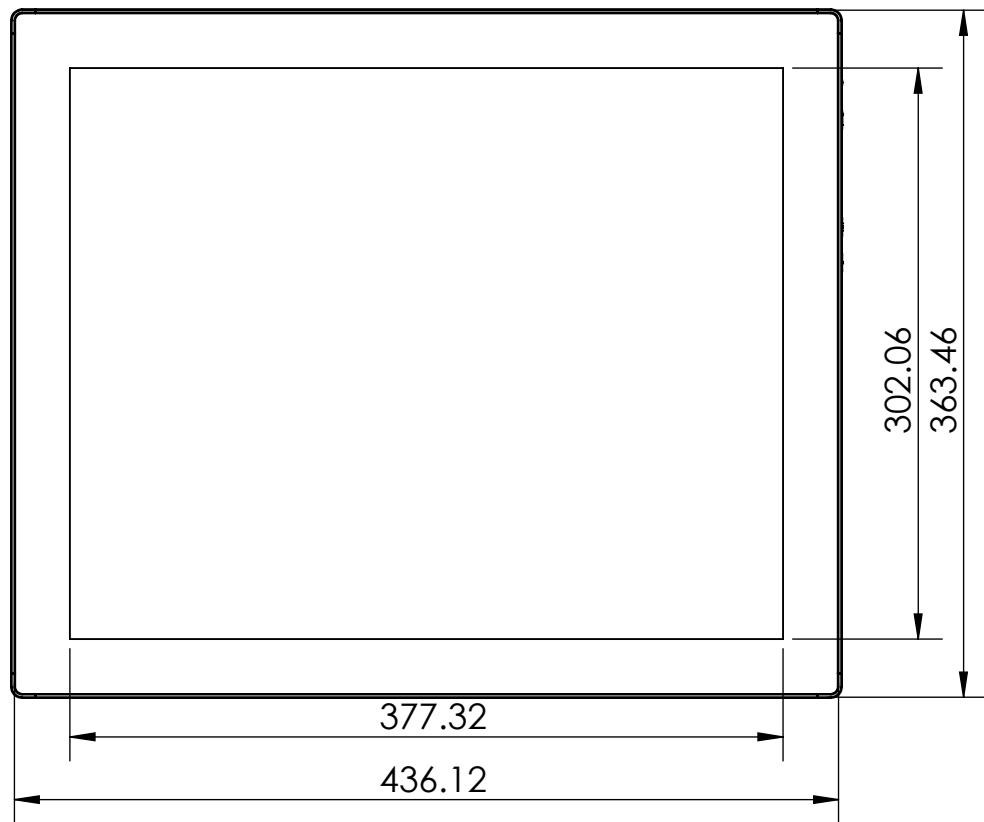
Bottom View
