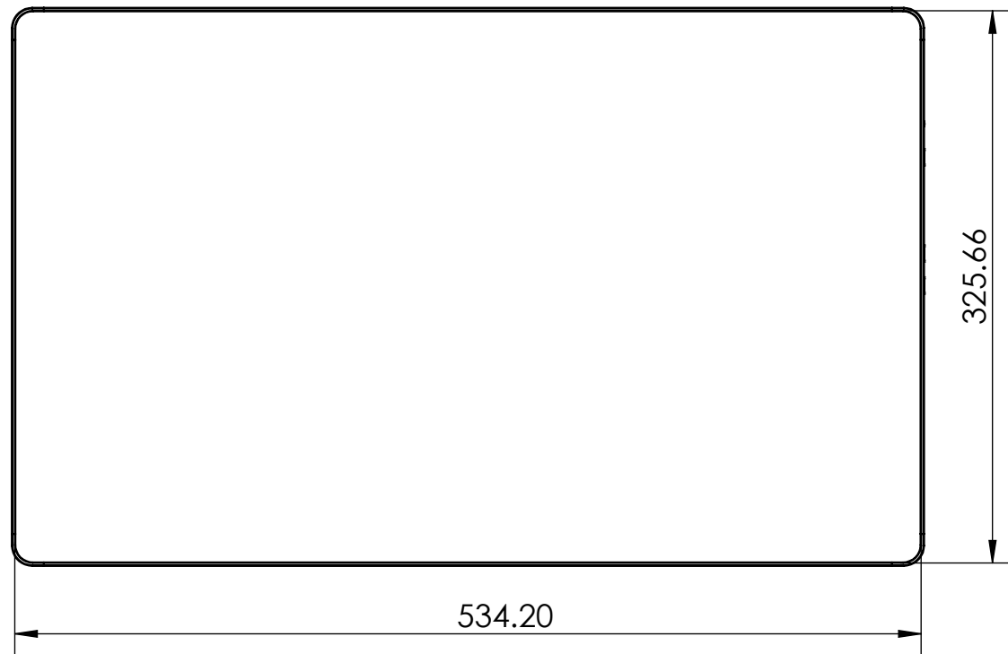
Bottom View
