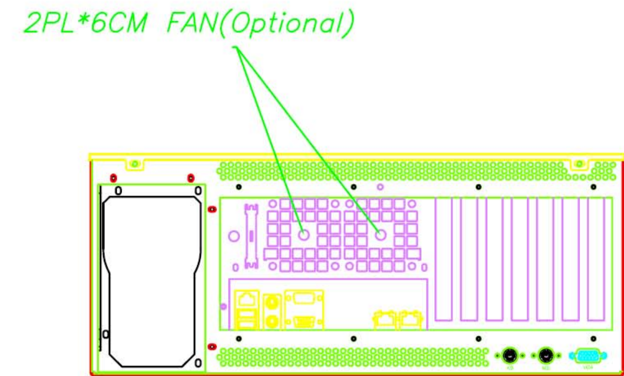
Rear View
