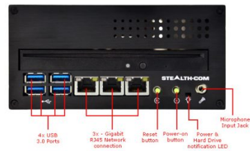
LPC-480PCIeG4 Front View
