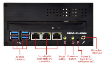
LPC-480PCIG4 Front View
