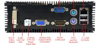
LPC-480G4FM Rear View
